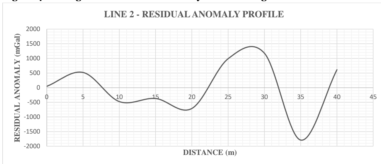
Figure 4.2f: Residual Anomaly Profile along Traverse 2
