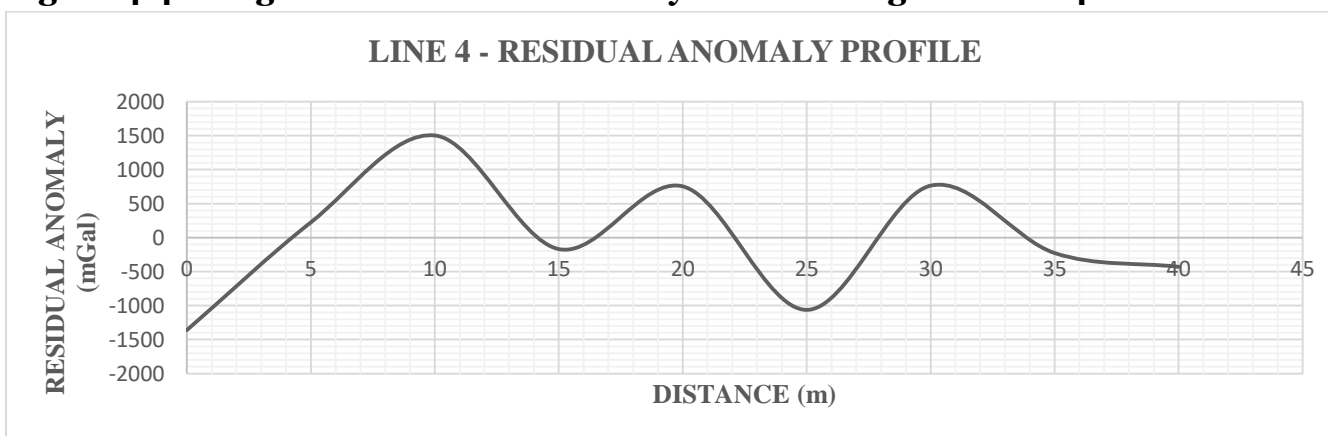
Figure 4.4f: Residual Anomaly Profile along Traverse 4
