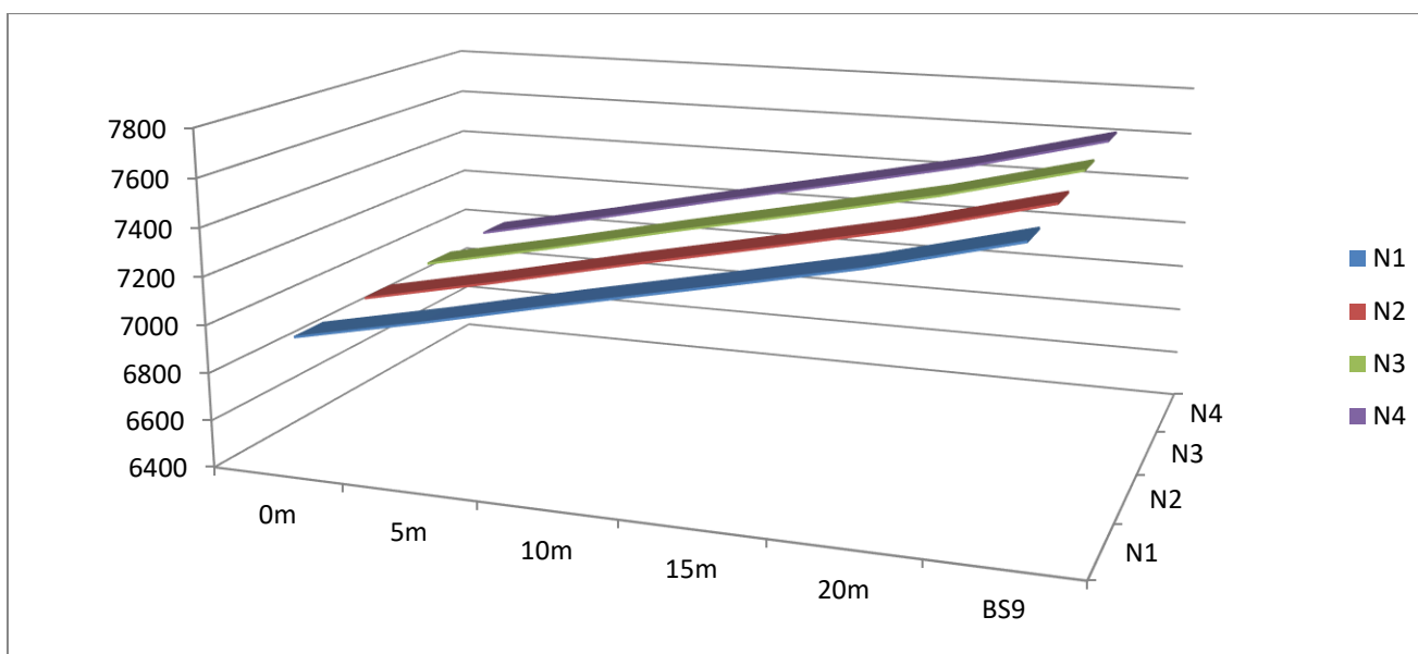
Figure 4.6b: Level of gravity changes in Igbeyin-Adun Area 1 line 5 using 3D lines
