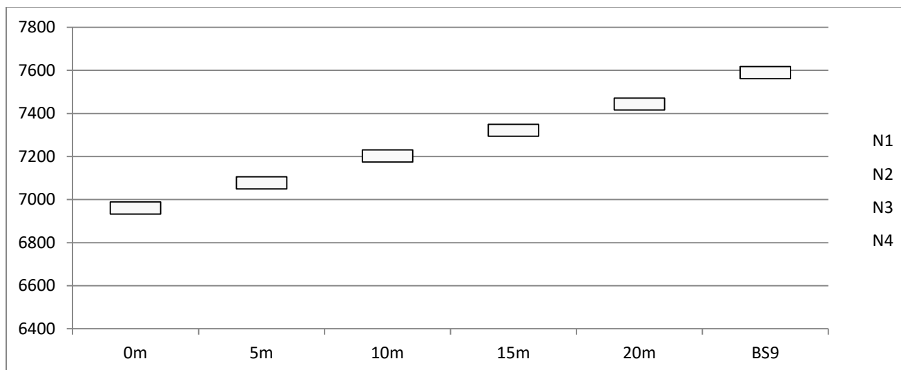
Figure 4.6c: High –Low close Description of gravity changes in Igbeyin-Adun Area 1 line1
