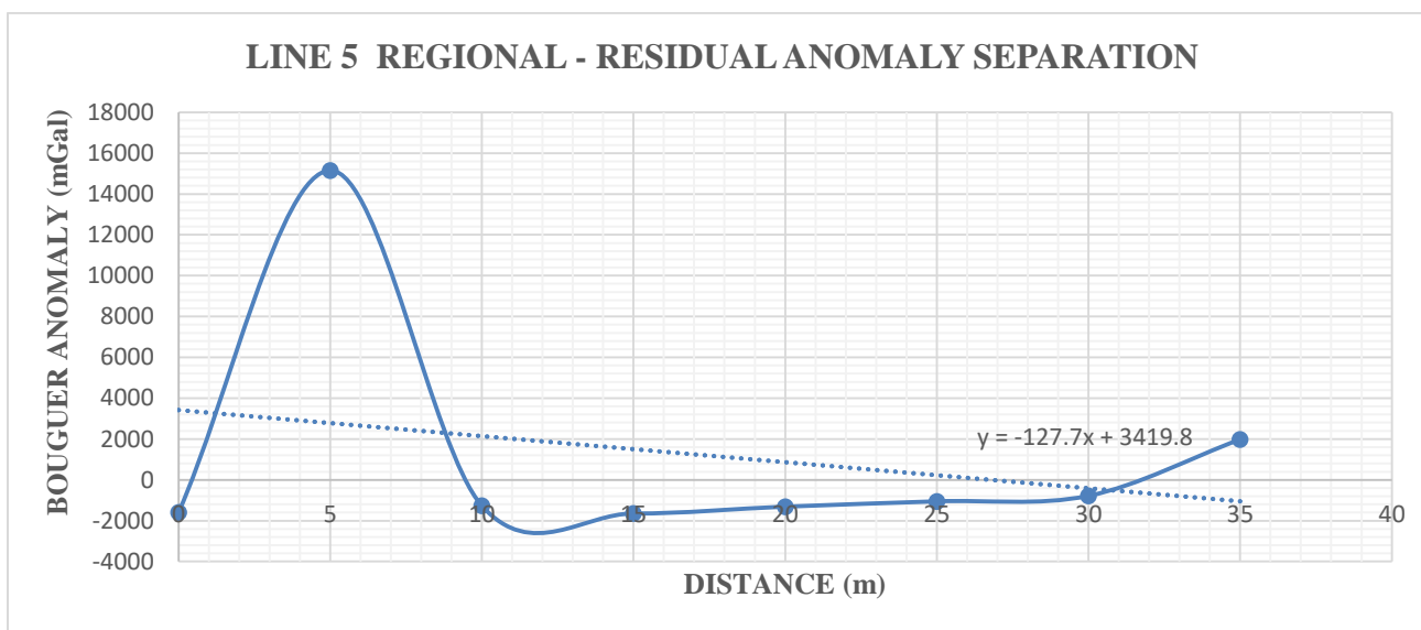
Figure 4.5e: Regional - Residual Anomaly Profile along Traverse 5
