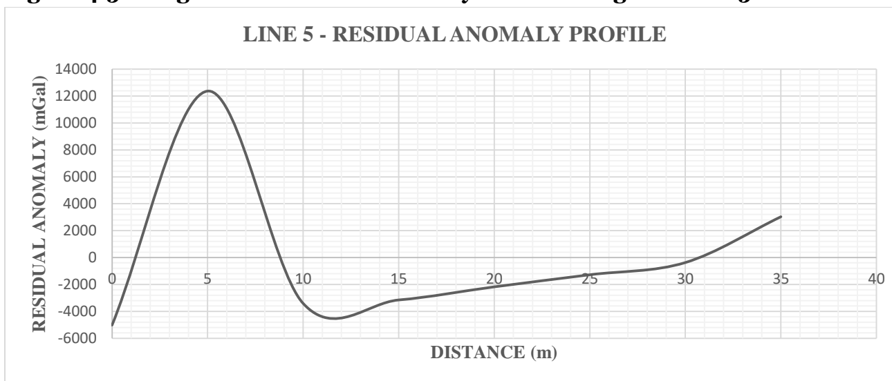
Figure 4.5f: Residual Anomaly Profile along Traverse 5
