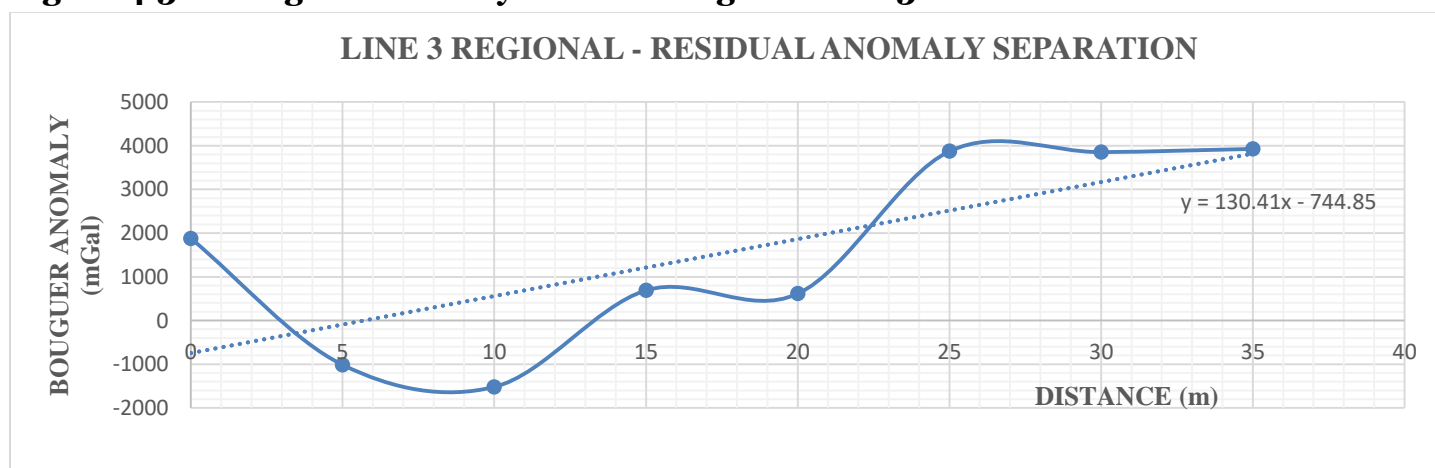
Figure 4.3e: Regional - Residual Anomaly Profile along Traverse 3
