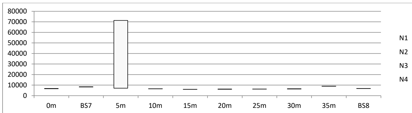
Figure 4.5c: High –Low close Description of gravity changes in Igbeyin-Adun Area 1 line1
