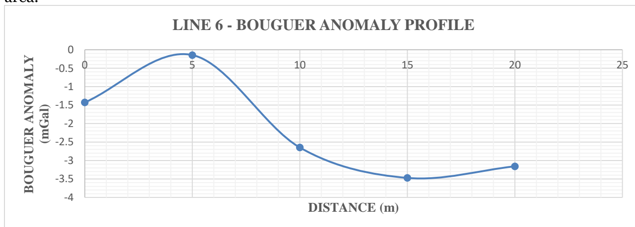
Figure 4.6d: Bouguer Anomaly Profile along Traverse 6
