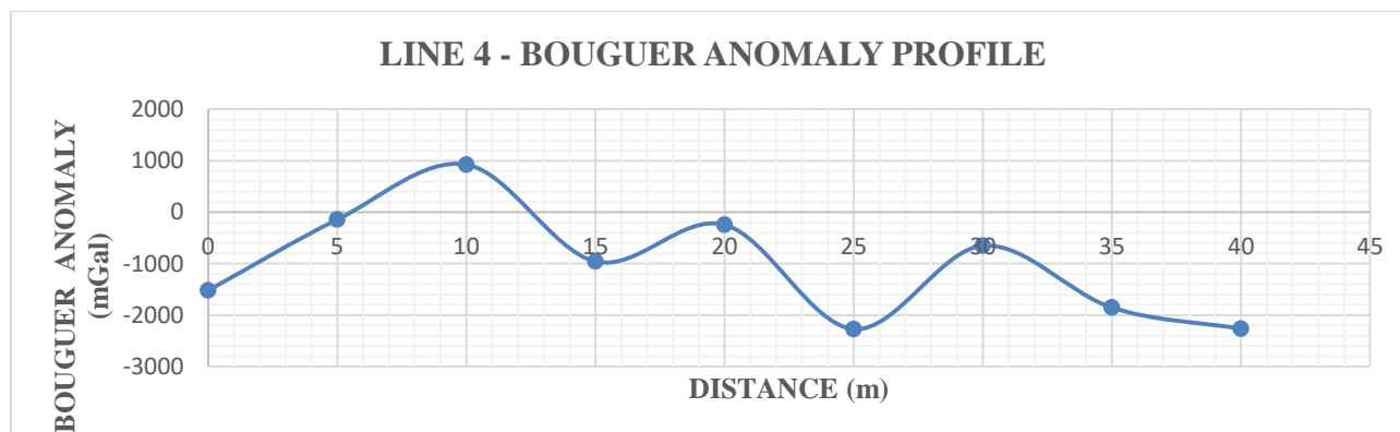
Figure 4.4d: Bouguer Anomaly Profile along Traverse 4
