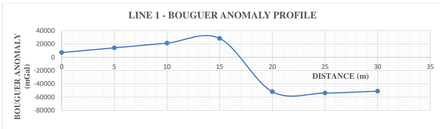
Figure 4.1d: Bouguer Anomaly Profile along Traverse 1
