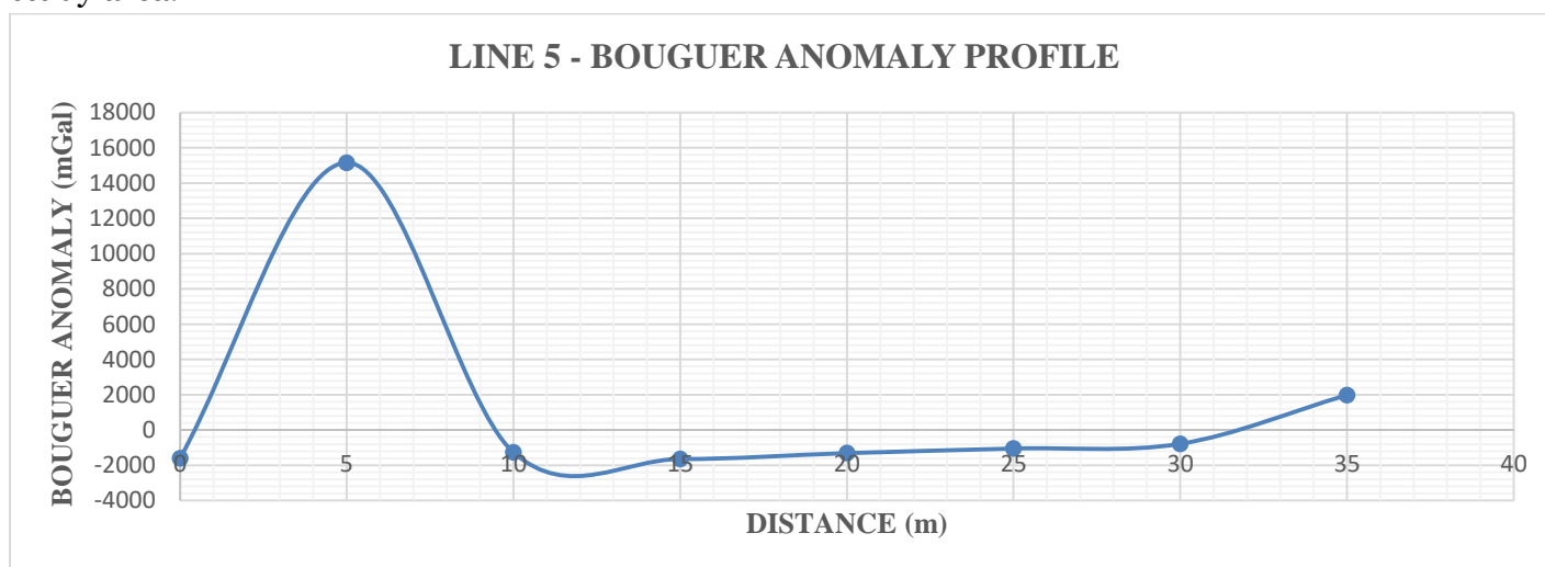
Figure 4.5d: Bouguer Anomaly Profile along Traverse 5
