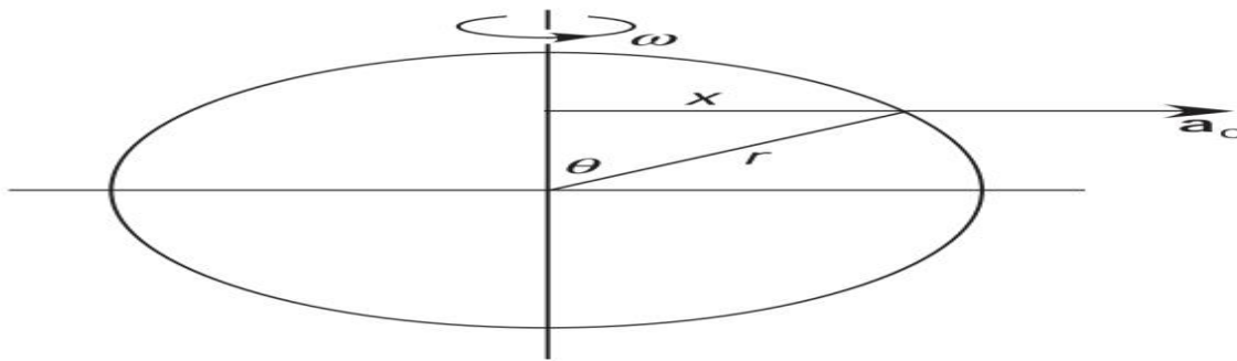
Fig. 3.2: Centrifugal acceleration a_c at co-latitude \theta , directed perpendicular to and away from the axis of rotation (Lowrie, 2011).
