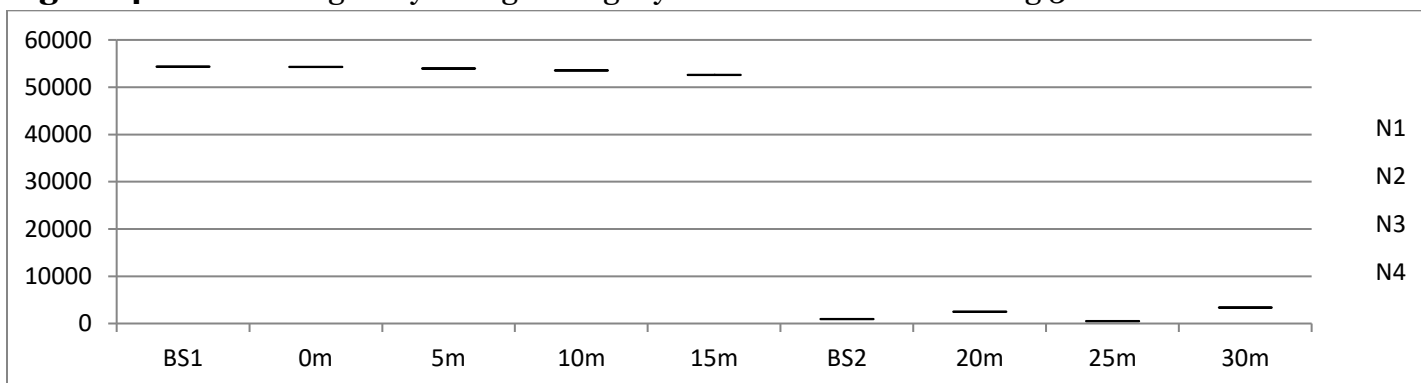
Figure 4.1c: High –Low close Description of gravity changes in Igbeyin-Adun Area 1 in line1
