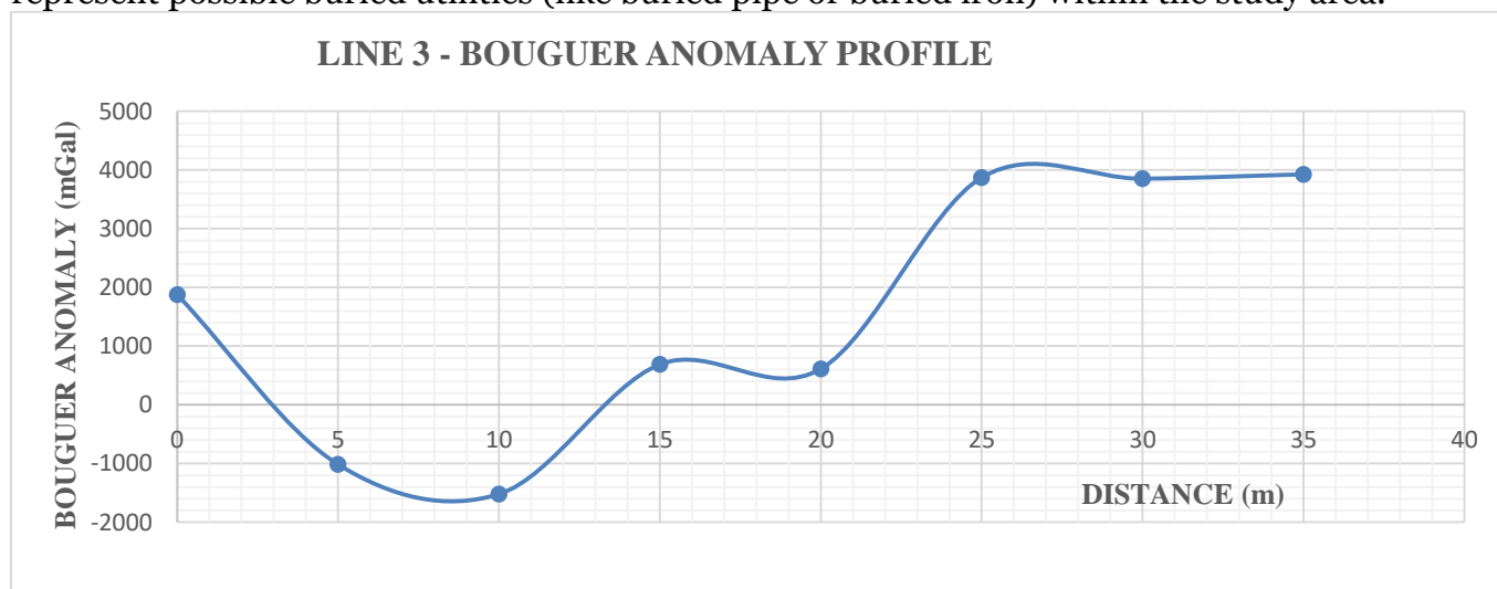
Figure 4.3d: Bouguer Anomaly Profile along Traverse 3
