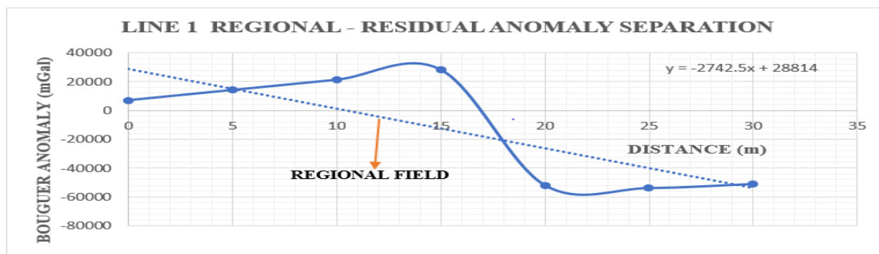
Figure 4.1e: Regional - Residual Anomaly Profile along Traverse 1
