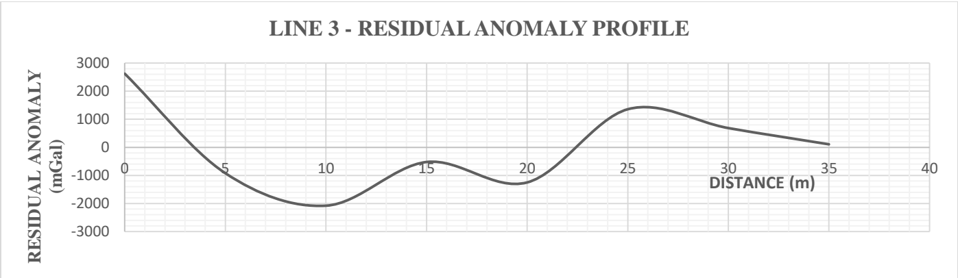
Figure 4.3f: Residual Anomaly Profile along Traverse3
