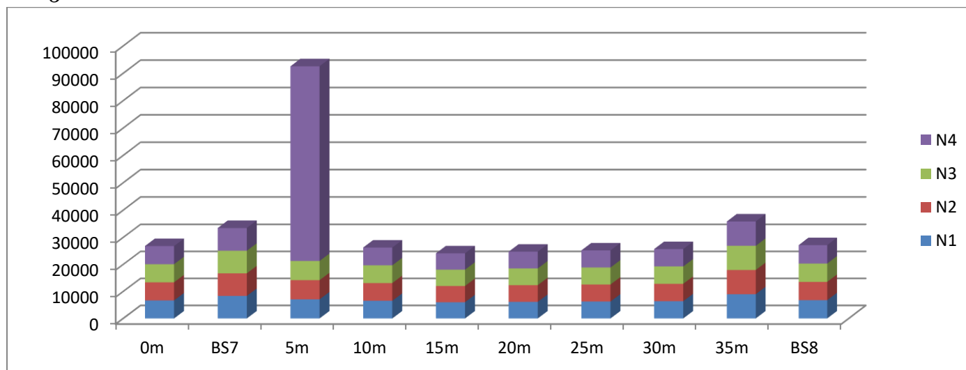
Figure 4.5a: Distribution of gravity changes in Igbeyin-Adun Area 1 line 5 using 3D Stacked Column
