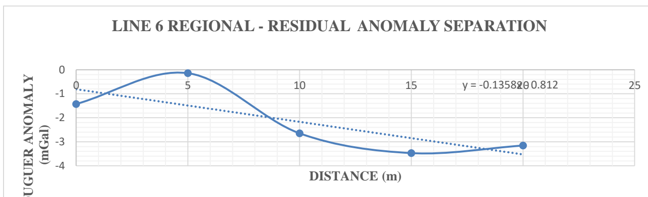
Figure 4.6e: Regional - Residual Anomaly Profile along Traverse 6
