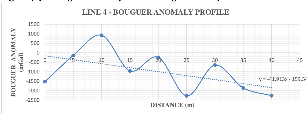
Figure 4.4e: Regional - Residual Anomaly Profile along Traverse 4
