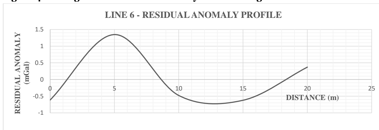
Figure 4.6c: Residual Anomaly Profile along Traverse 6
