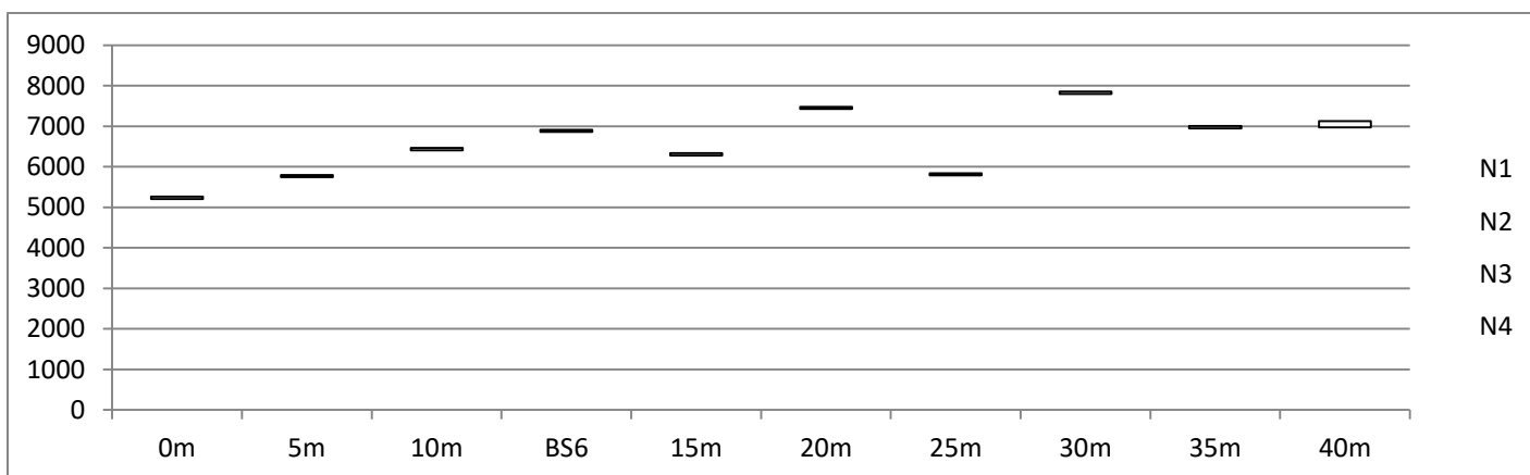
Figure 4.4c: High–Low close Description of gravity changes in Igbeyin-Adun Area 1 line 4
