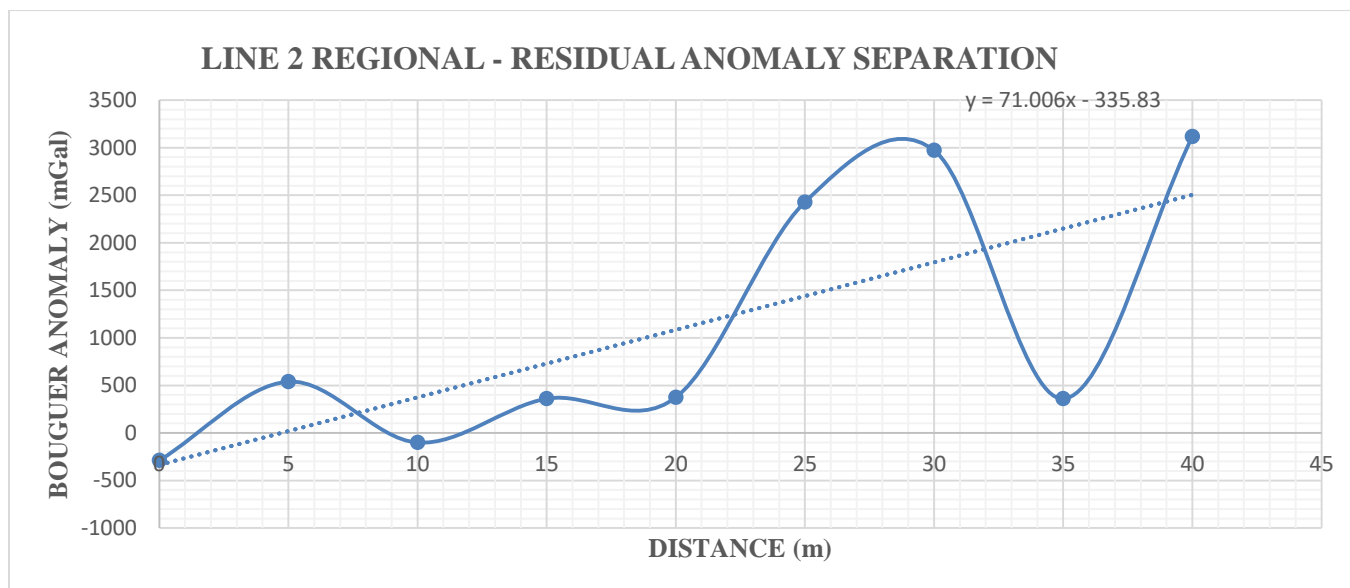
Figure 4.2e: Regional - Residual Anomaly Profile along Traverse 2
