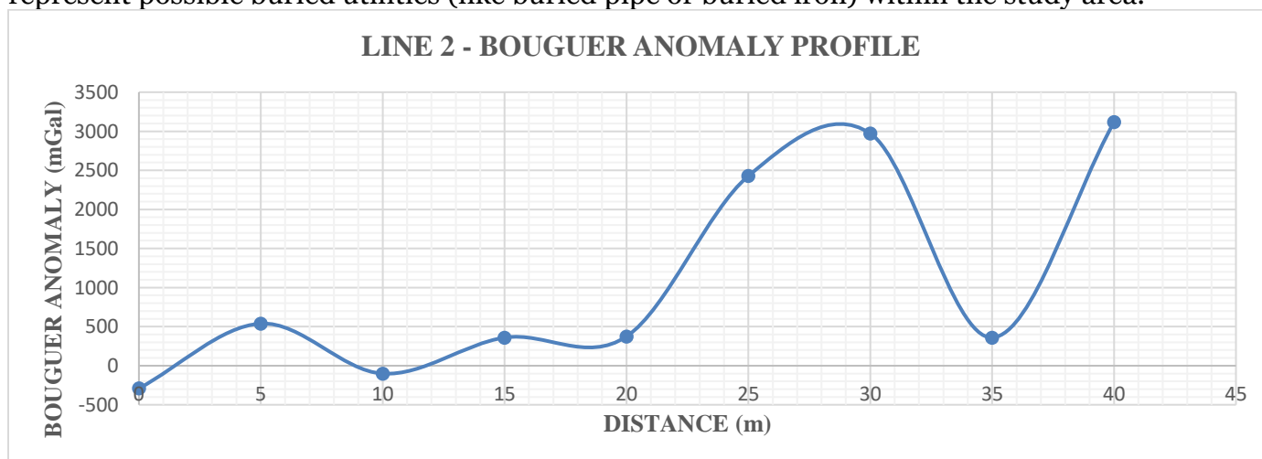
Figure 4.2d: Bouguer Anomaly Profile along Traverse 2
