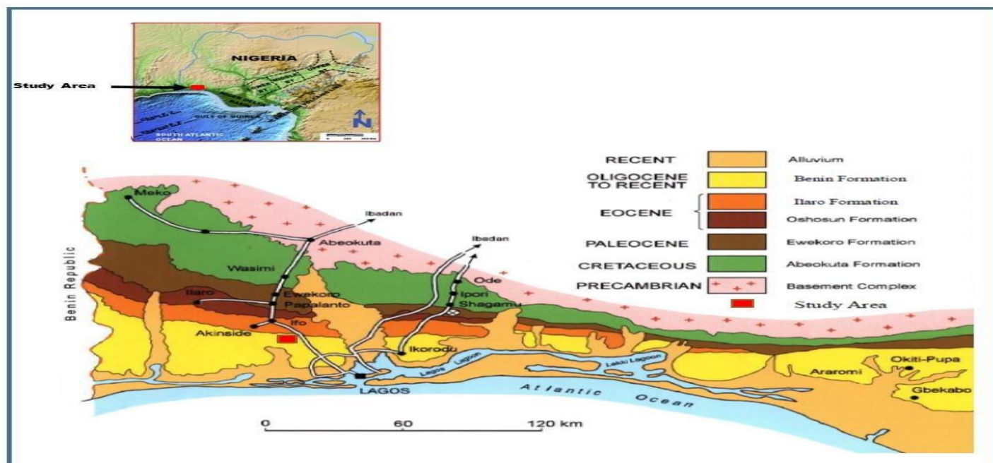
Figure 2.1: Stratigraphic of Eastern Dahomey Basin Southwestern Nigeria (Bakare et al. , 2019)
