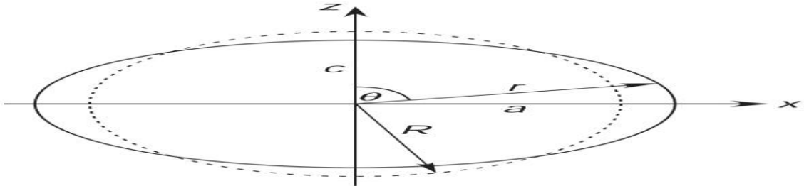
Fig. 3.1: Polar cross-section of a spheroid with principal axes a and c ( c < a ), compared with a sphere (dashed) with radius R and the same volume as spheroid (Lowrie, 2011).
