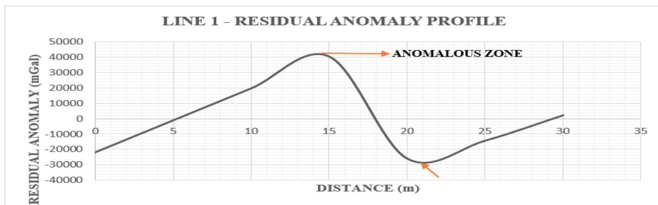
Figure 4.1f: Residual Anomaly Profile along Traverse 1
